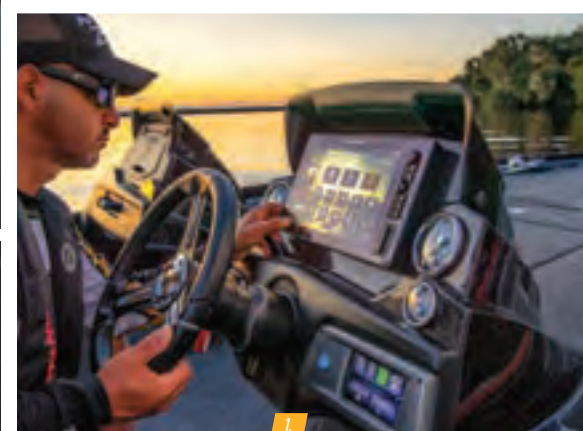
1. NEW modular, aerodynamic console design w/expanded leg clearance & larger graph surface 2. Massive, lockable center bow tackle storage w/molded-in rain/spray channels, dual piston lift assist, LED lighting & optional magnetic under-lid lure organizer. 3. Oversized, lockable bow port & starboard rod lockers w/lift assists for rods up to 8' (2.44 m)
