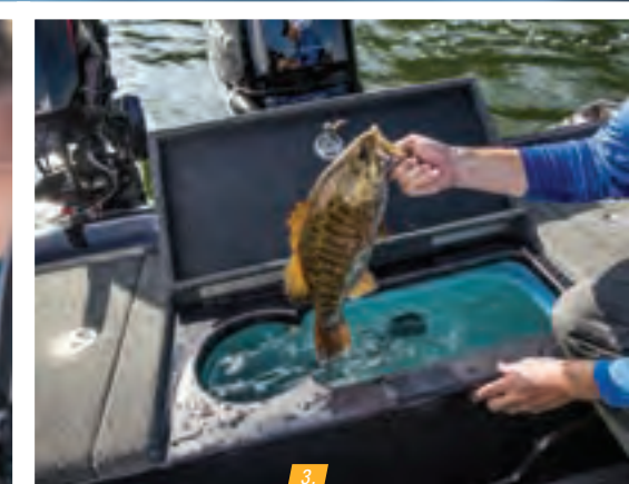
1. NEW touchscreen switch panel w/1-touch boat controls including First Fish, Nite Mode, master power, trim, lighting, bilge, livewells & more 2. 3-level center rod locker for rods up to 8' (2.44 m) w/tapered rod tubes to protect rod tips 3. Aft 26-gal. (98.42 L) GUARDIAN™, anti-slosh livewell & bow 5.5-gal. (20.82 L) baitwell w/bucket
